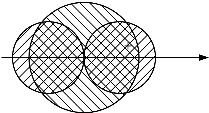
Fig. 21-11 Hybridization of s and p orbitals
