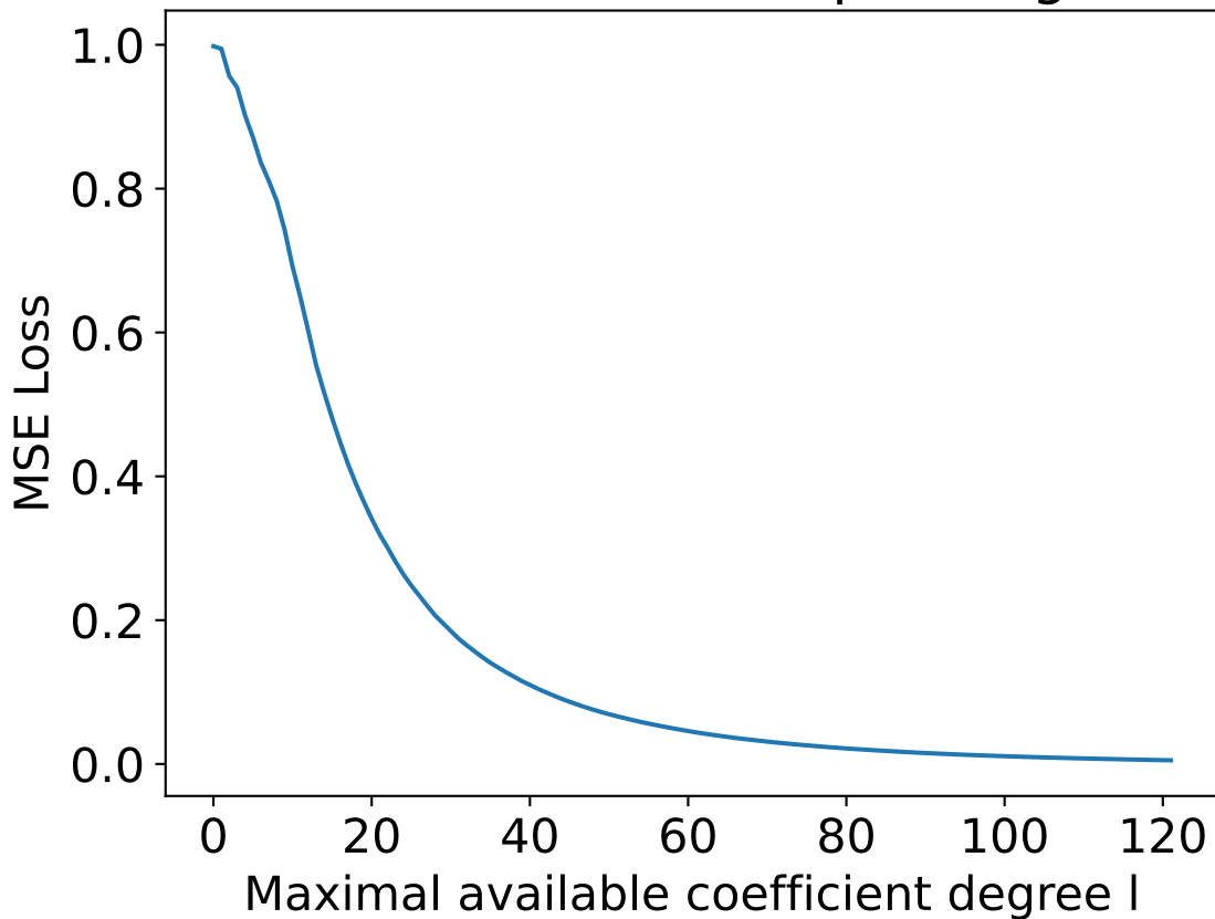
MSE Loss of reconstruction of wind speed maps from SH coefficients up to degree l
