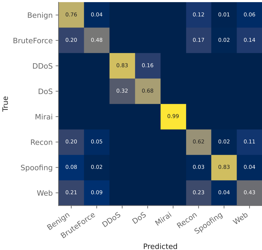
DistilBERT confusion, row-normalized mean of three seeds
