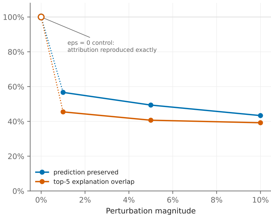
Degradation from a zero noise floor
