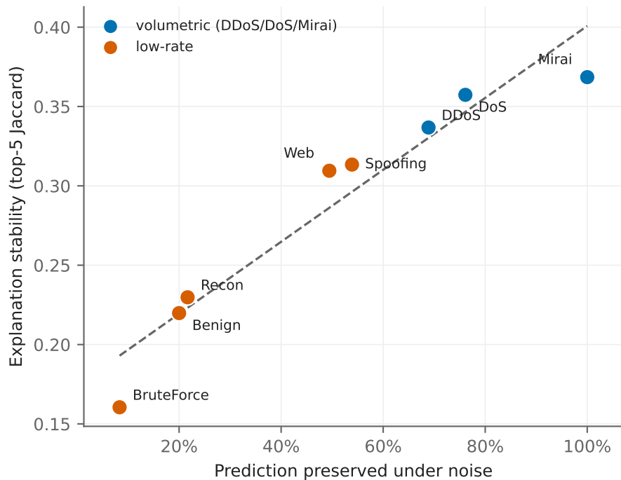
Explanation stability tracks decision stability ( r = +0.96 )
