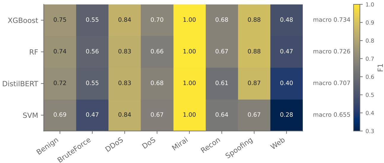
Per-class F1 by model (CICIoT2023 test)
