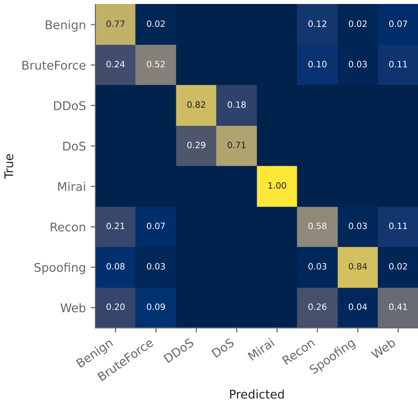
DistilBERT confusion (row-normalized)
