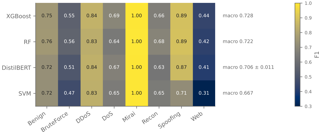
Per-class F1 by model (CICIoT2023 test)
