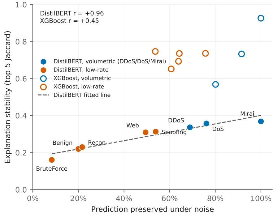
Per-class coupling is encoder-specific
