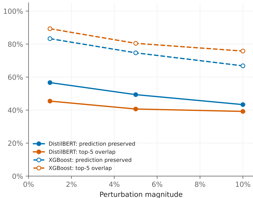
Degradation under the same perturbation
