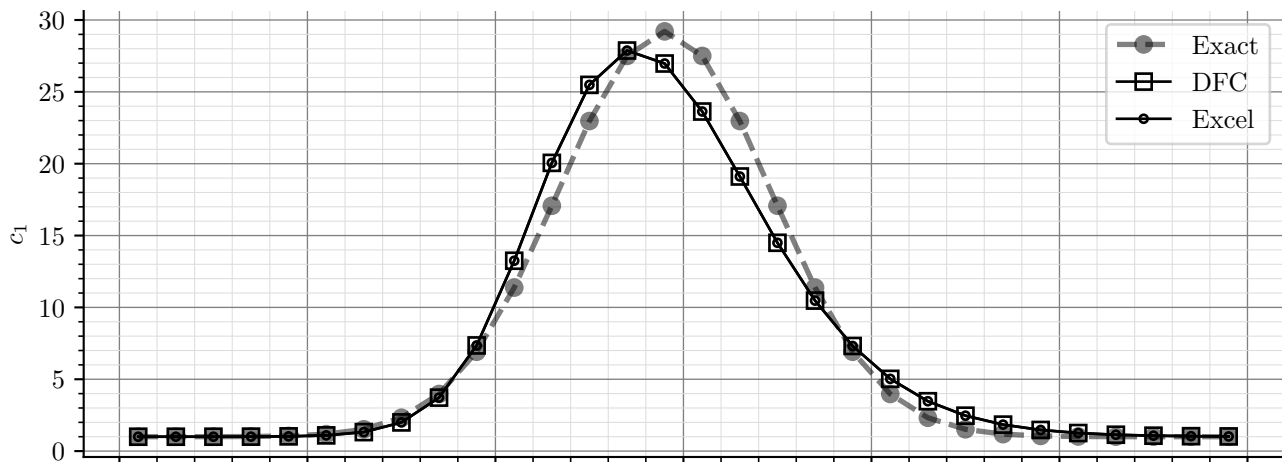
Species concentration, t = 10 days
