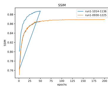
Figure 27: * SSIM
