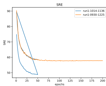
Figure 29: * SRE
