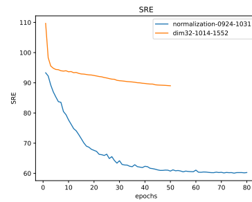
Figure 5: * SRE
