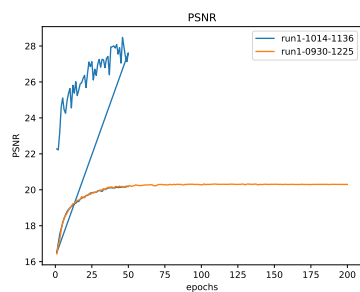
Figure 26: * PSNR
