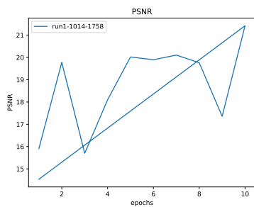
Figure 46: * PSNR
