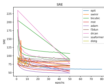
Figure 54: * SRE
