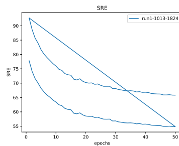
Figure 24: * SRE
