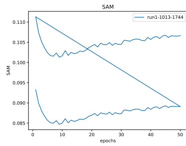
Figure 33: * SAM
