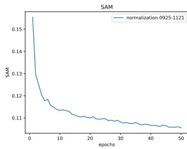
Figure 43: * SAM
