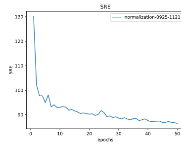
Figure 44: * SRE
