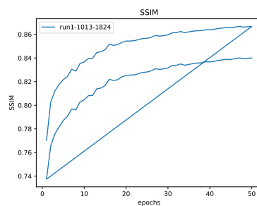
Figure 22: * SSIM
