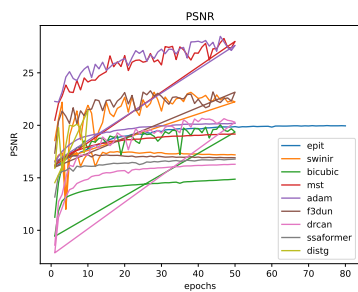
Figure 51: * PSNR
