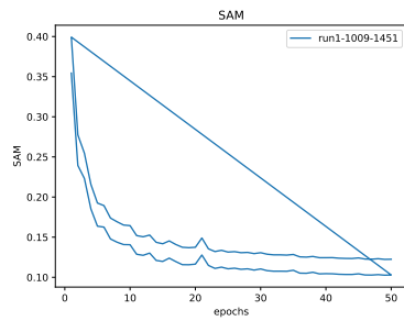
Figure 38: * SAM
