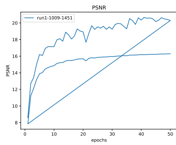
Figure 36: * PSNR
