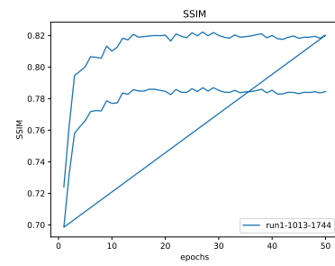
Figure 32: * SSIM
