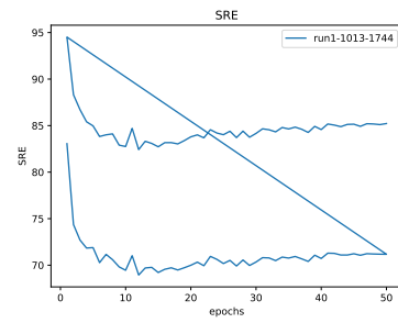
Figure 34: * SRE
