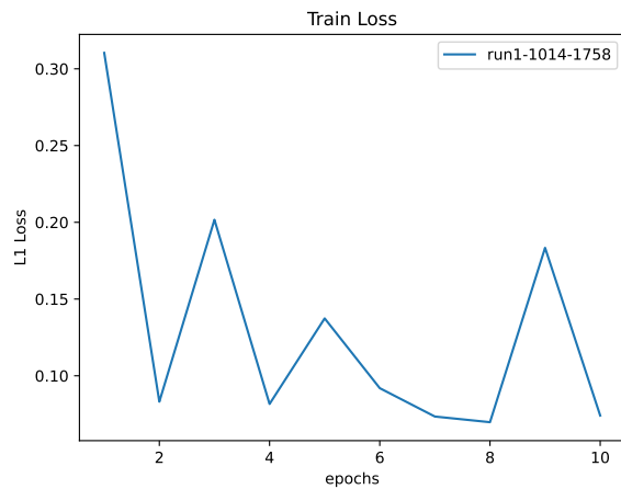
Figure 45: Train Loss
