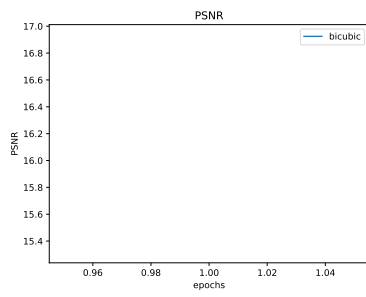
Figure 11: * PSNR
