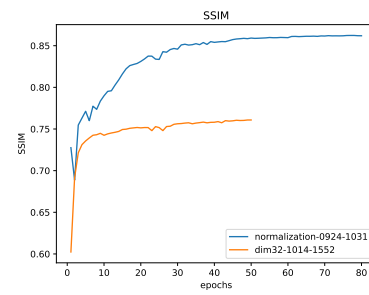
Figure 3: * SSIM
