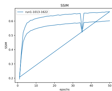
Figure 17: * SSIM
