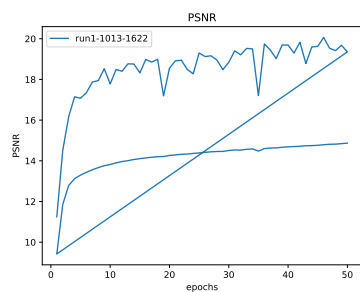
Figure 16: * PSNR
