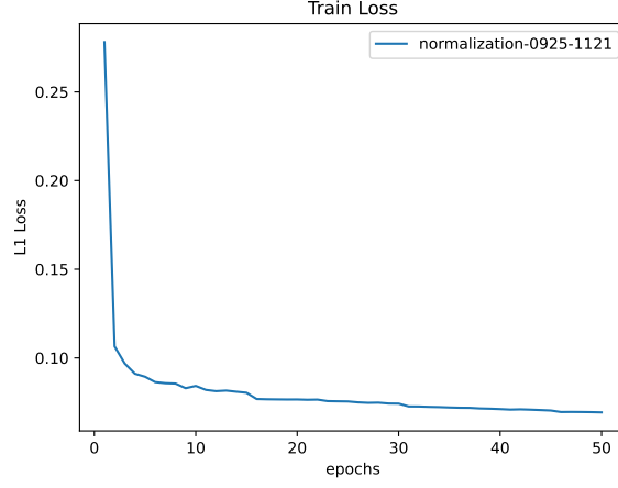
Figure 40: Train Loss
