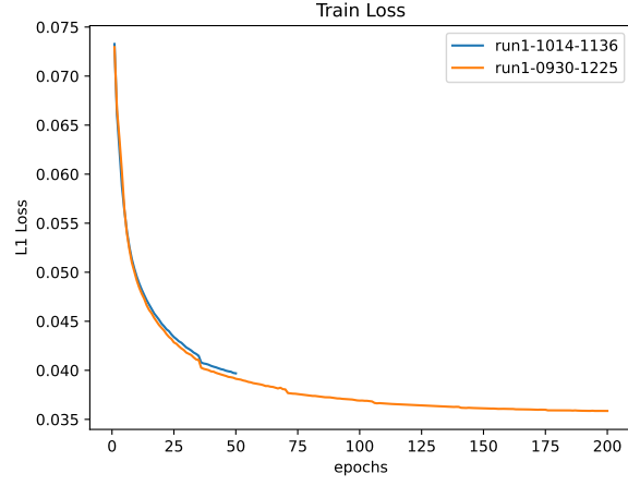
Figure 25: Train Loss
