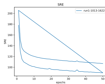
Figure 19: * SRE
