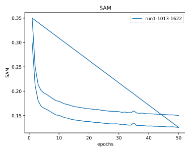
Figure 18: * SAM
