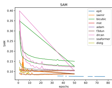
Figure 53: * SAM
