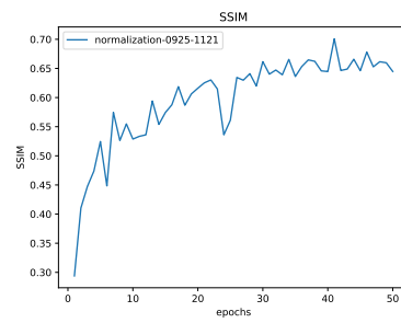
Figure 42: * SSIM
