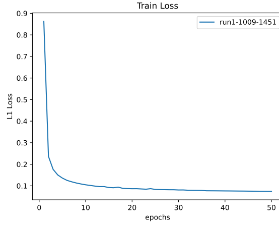
Figure 35: Train Loss
