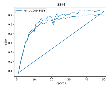
Figure 37: * SSIM
