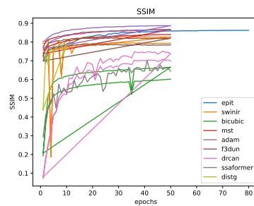
Figure 52: * SSIM
