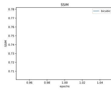
Figure 12: * SSIM
