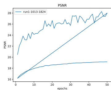
Figure 21: * PSNR
