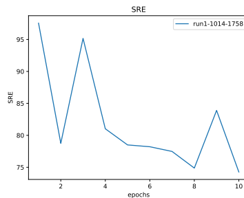
Figure 49: * SRE
