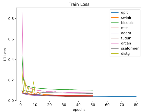
Figure 50: Train Loss
