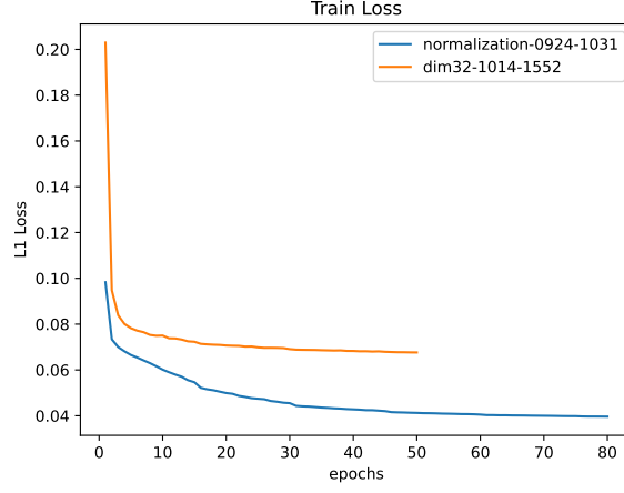
Figure 1: Train Loss
