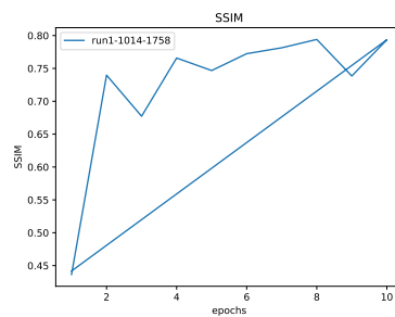
Figure 47: * SSIM
