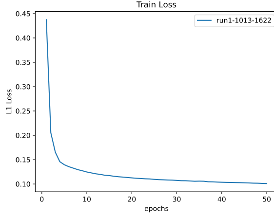
Figure 15: Train Loss
