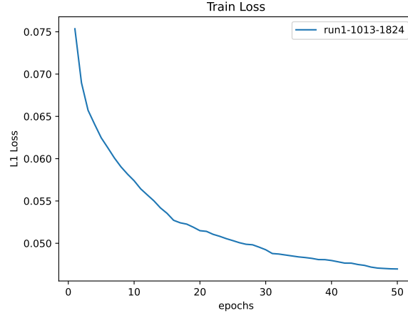
Figure 20: Train Loss
