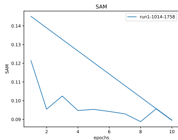
Figure 48: * SAM
