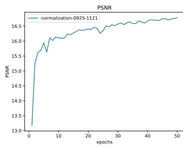
Figure 41: * PSNR
