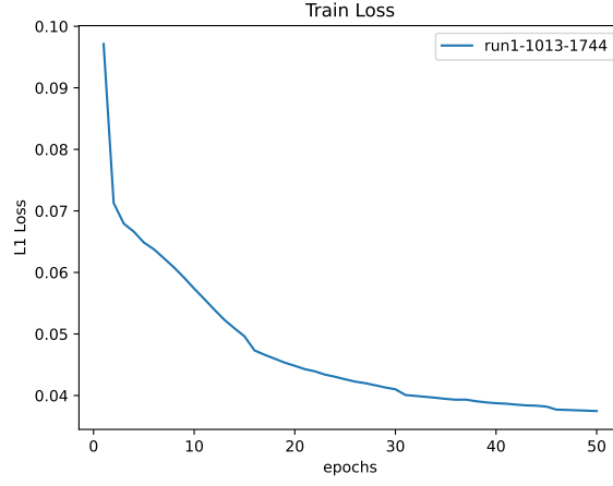
Figure 30: Train Loss
