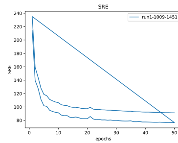
Figure 39: * SRE
