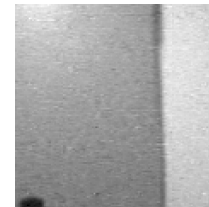
distg_unet
