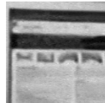
distg_unet
