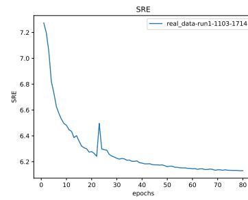
Figure 45: * SRE
