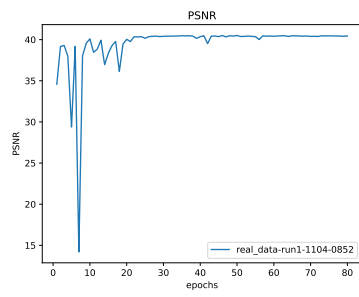
Figure 17: * PSNR
