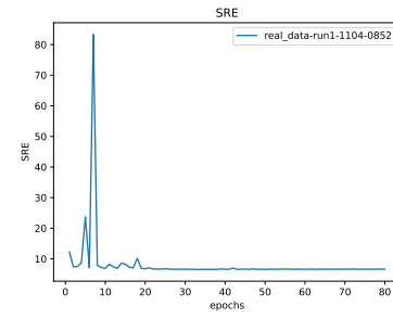
Figure 20: * SRE
