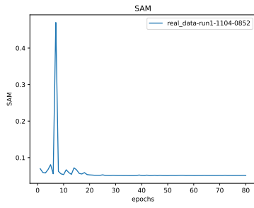
Figure 19: * SAM
