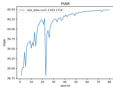
Figure 42: * PSNR
