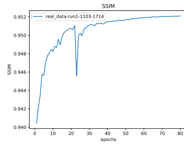
Figure 43: * SSIM
