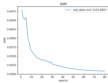
Figure 14: * SAM
