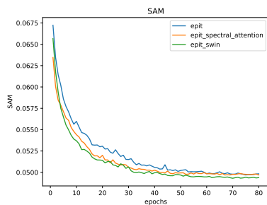
Figure 54: * SAM
