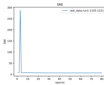
Figure 30: * SRE
