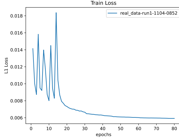
Figure 16: Train Loss
