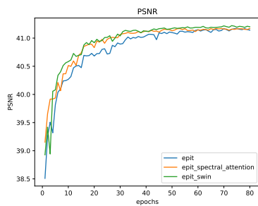
Figure 52: * PSNR
