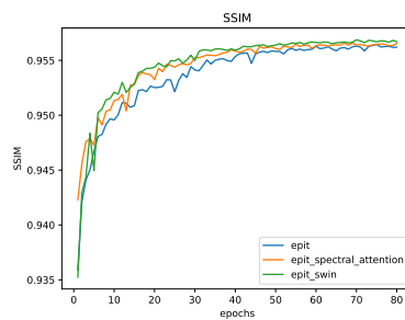
Figure 53: * SSIM
