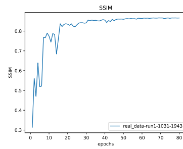
Figure 3: * SSIM
