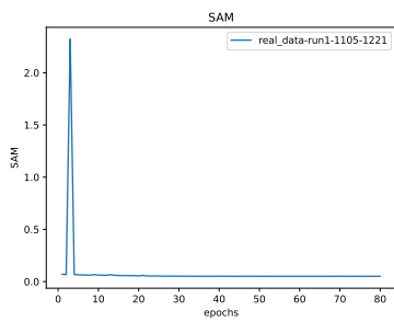
Figure 29: * SAM
