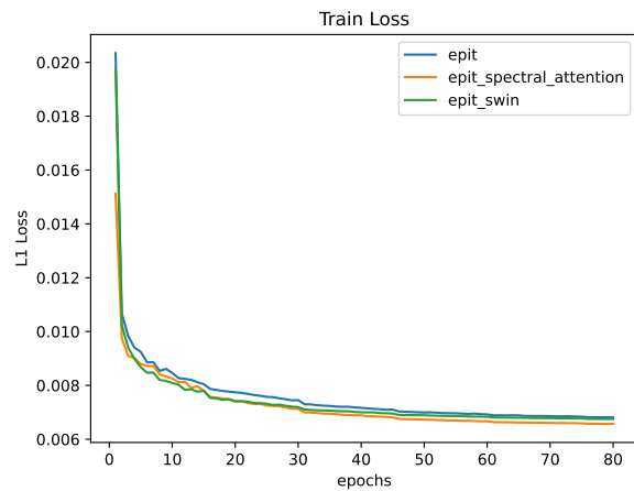
Figure 51: Train Loss
