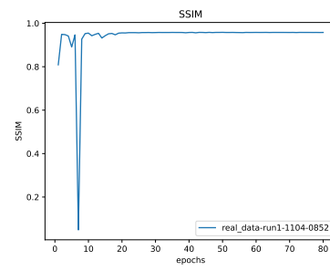
Figure 18: * SSIM
