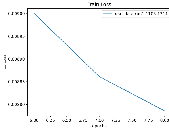
Figure 41: Train Loss
