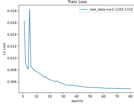
Figure 21: Train Loss
