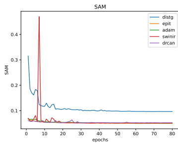
Figure 29: * SAM
