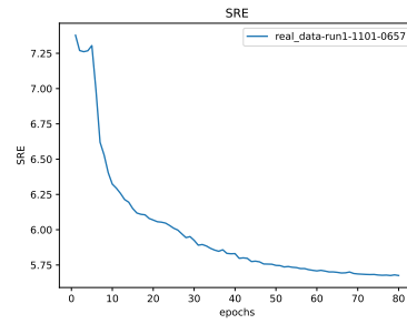
Figure 15: * SRE
