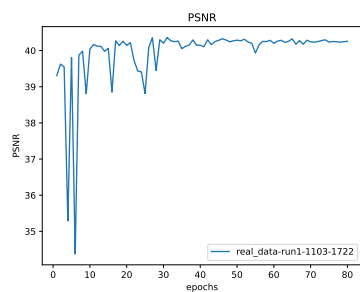
Figure 22: * PSNR
