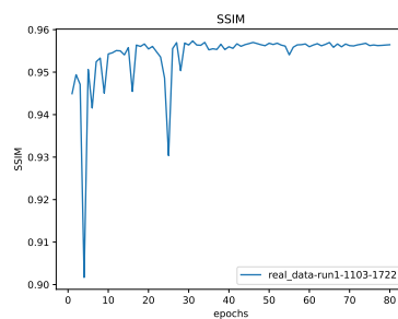
Figure 23: * SSIM
