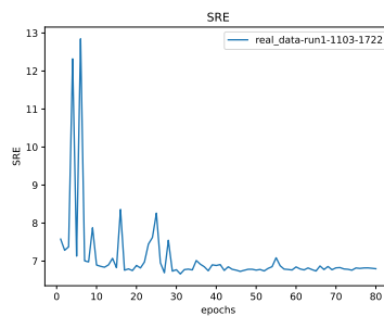
Figure 25: * SRE
