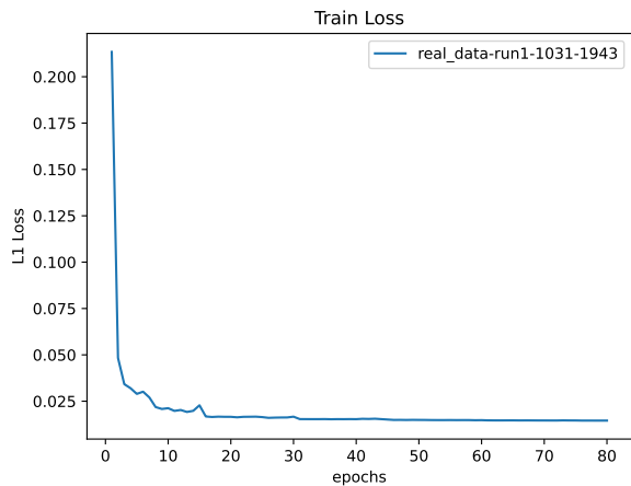
Figure 1: Train Loss
