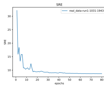
Figure 5: * SRE
