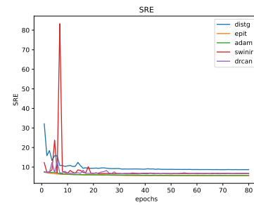
Figure 30: * SRE
