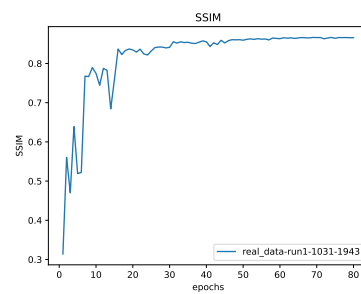
Figure 3: * SSIM
