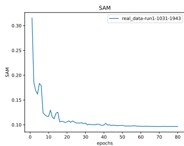
Figure 4: * SAM
