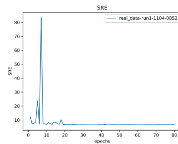
Figure 20: * SRE
