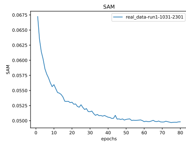
Figure 9: * SAM
