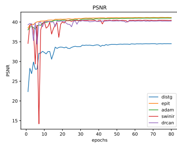
Figure 27: * PSNR
