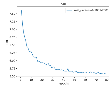
Figure 10: * SRE
