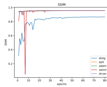
Figure 28: * SSIM
