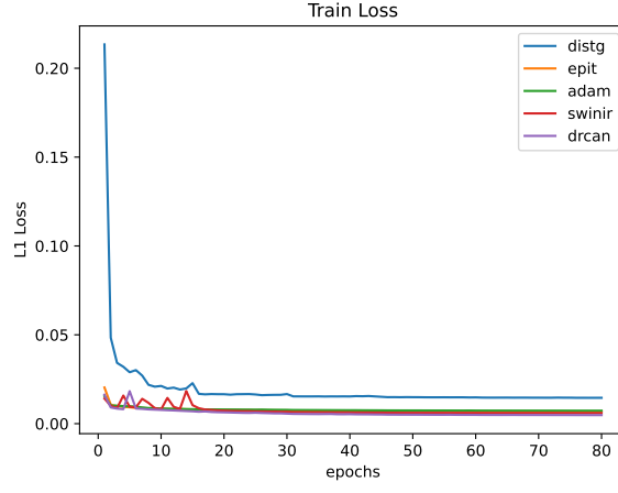
Figure 26: Train Loss
