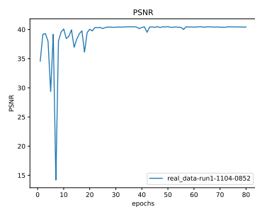
Figure 17: * PSNR
