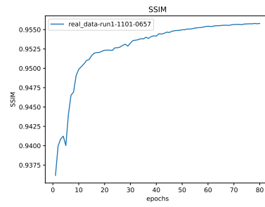
Figure 13: * SSIM
