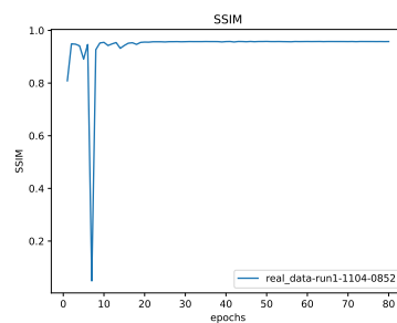
Figure 18: * SSIM
