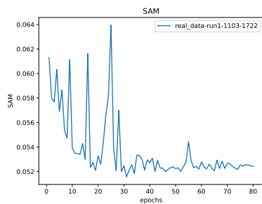
Figure 24: * SAM
