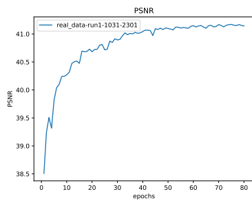
Figure 7: * PSNR
