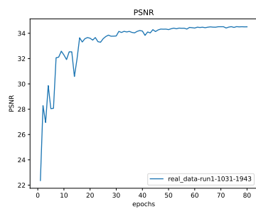
Figure 2: * PSNR
