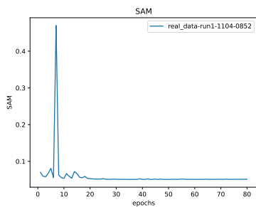
Figure 19: * SAM
