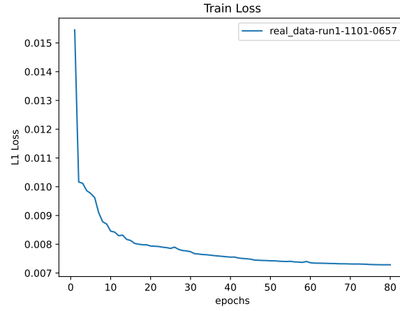
Figure 11: Train Loss
