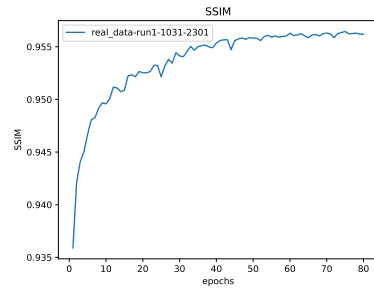
Figure 8: * SSIM
