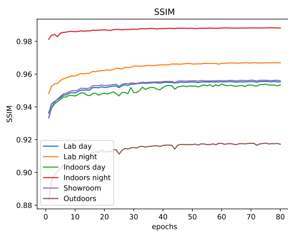
Figure 4: SSIM
