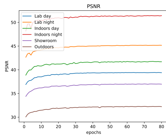
Figure 3: PSNR
