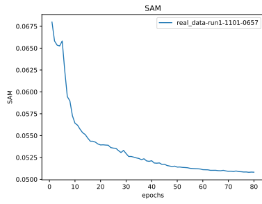
Figure 14: * SAM
