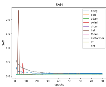
Figure 54: * SAM
