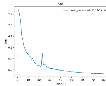
Figure 45: * SRE
