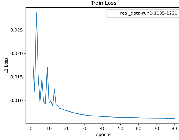
Figure 26: Train Loss
