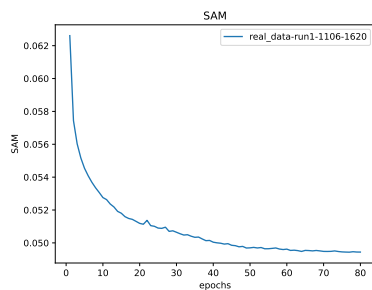
Figure 49: * SAM
