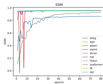
Figure 53: * SSIM
