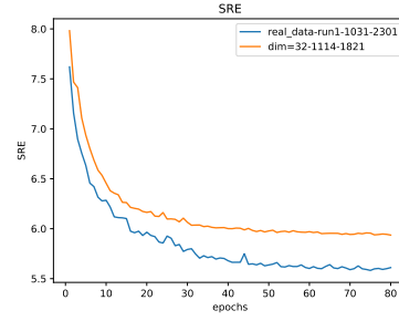
Figure 10: * SRE
