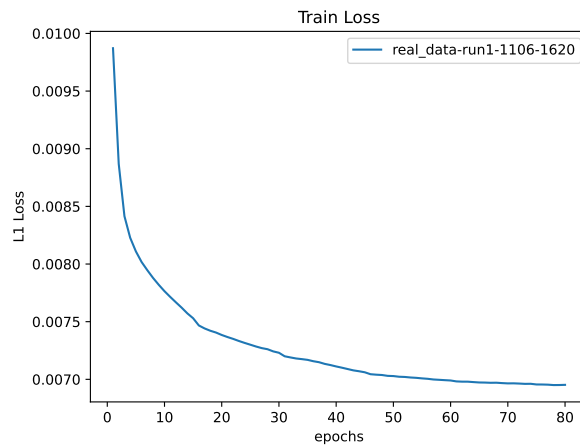
Figure 46: Train Loss
