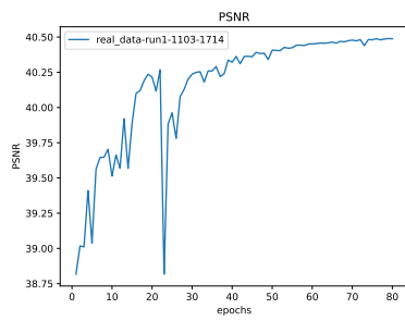
Figure 42: * PSNR
