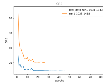
Figure 5: * SRE
