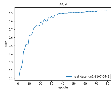
Figure 38: * SSIM
