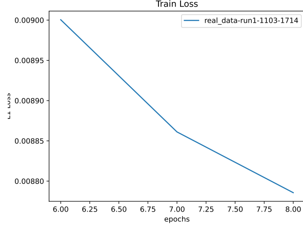
Figure 41: Train Loss
