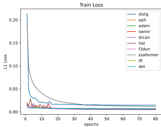
Figure 51: Train Loss
