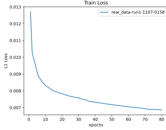
Figure 31: Train Loss
