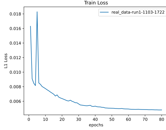
Figure 21: Train Loss
