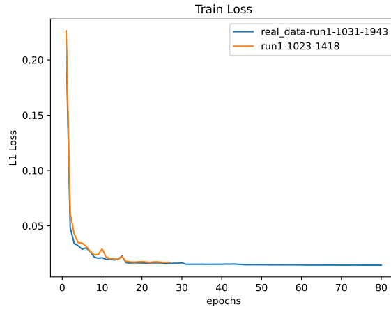
Figure 1: Train Loss
