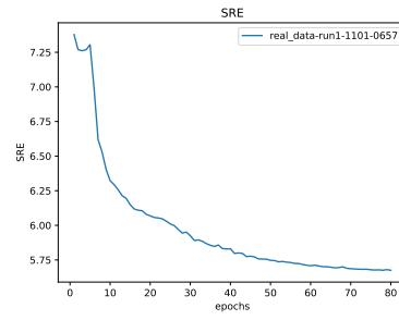
Figure 15: * SRE
