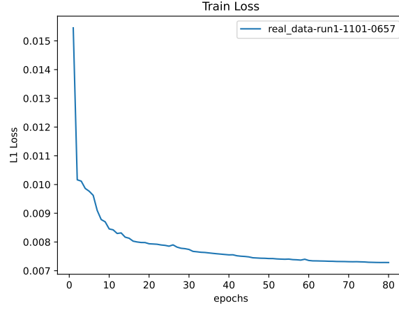
Figure 11: Train Loss
