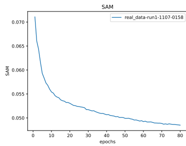
Figure 34: * SAM
