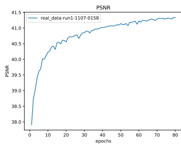
Figure 32: * PSNR
