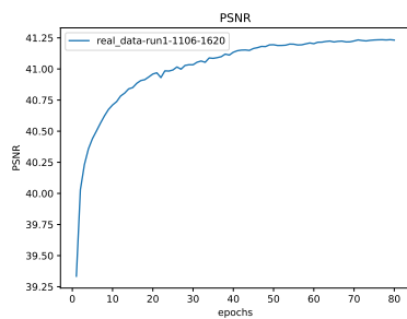
Figure 47: * PSNR
