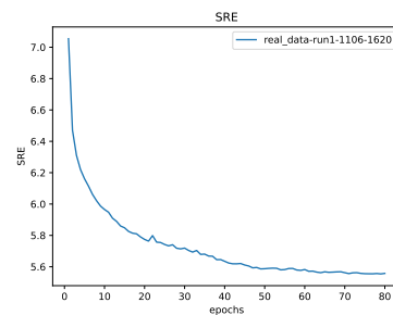
Figure 50: * SRE
