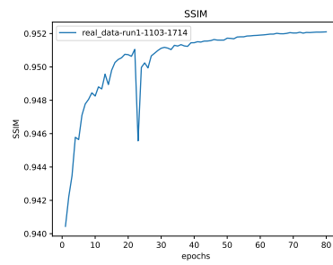
Figure 43: * SSIM
