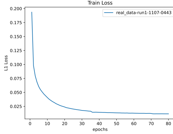
Figure 36: Train Loss
