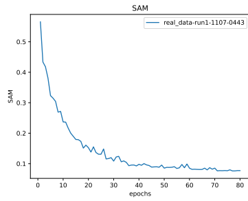
Figure 39: * SAM
