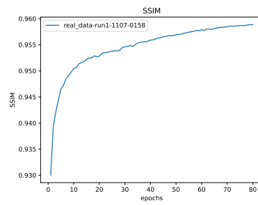
Figure 33: * SSIM
