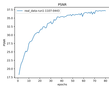
Figure 37: * PSNR
