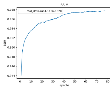
Figure 48: * SSIM
