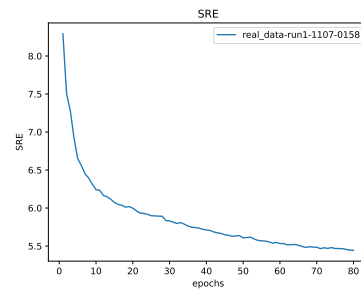
Figure 35: * SRE
