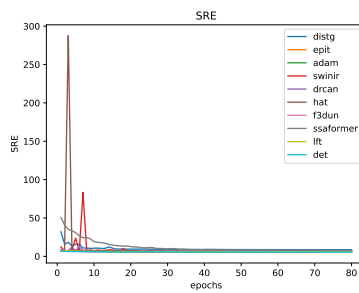
Figure 55: * SRE
