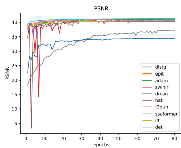
Figure 52: * PSNR
