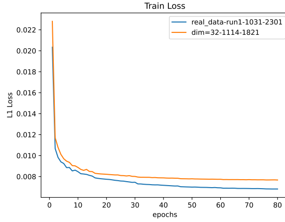
Figure 6: Train Loss
