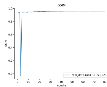
Figure 28: * SSIM
