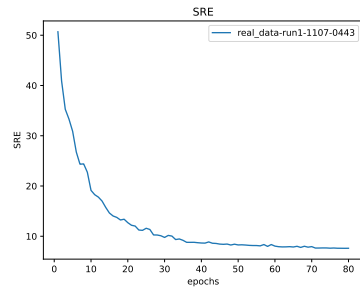
Figure 40: * SRE
