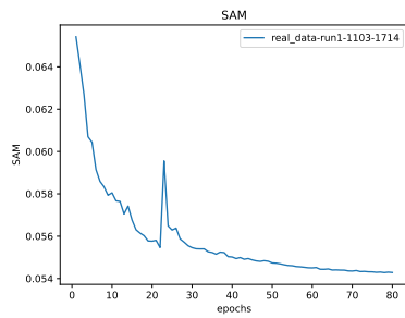
Figure 44: * SAM
