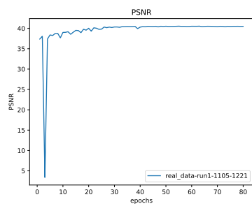
Figure 27: * PSNR
