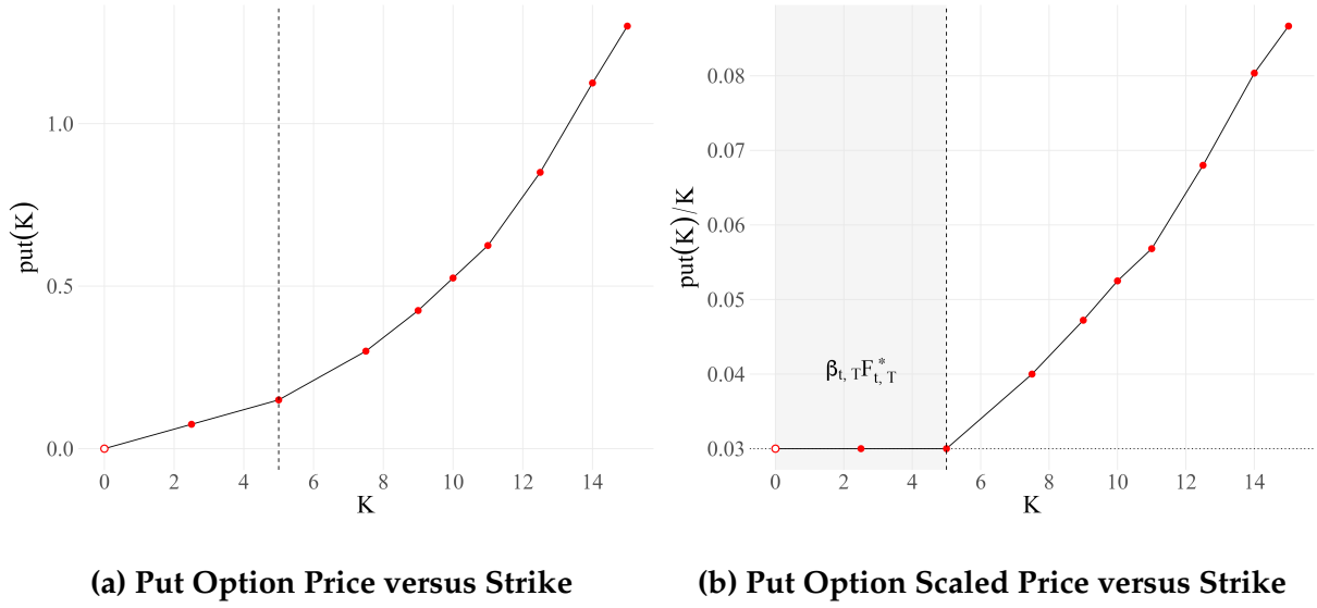
Figure 1: Put Option Price and Put Option Scaled Price Curves
