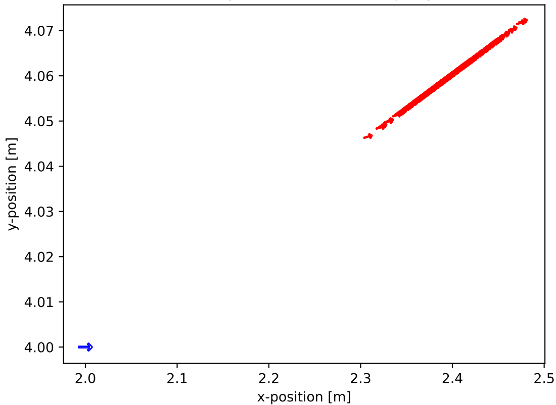
velocity motion model sampling
