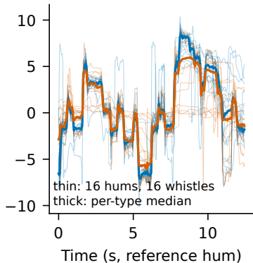
(c) 8 performers
