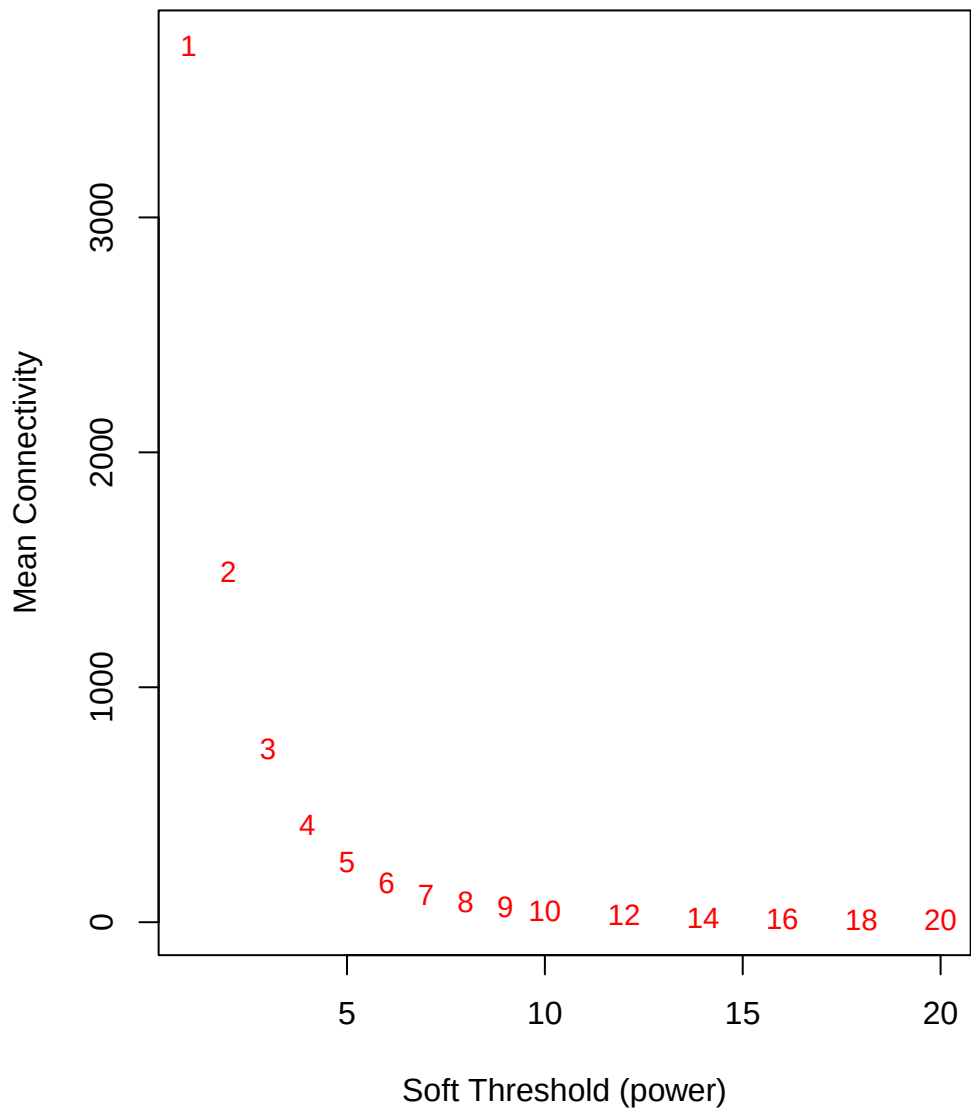
Mean connectivity
