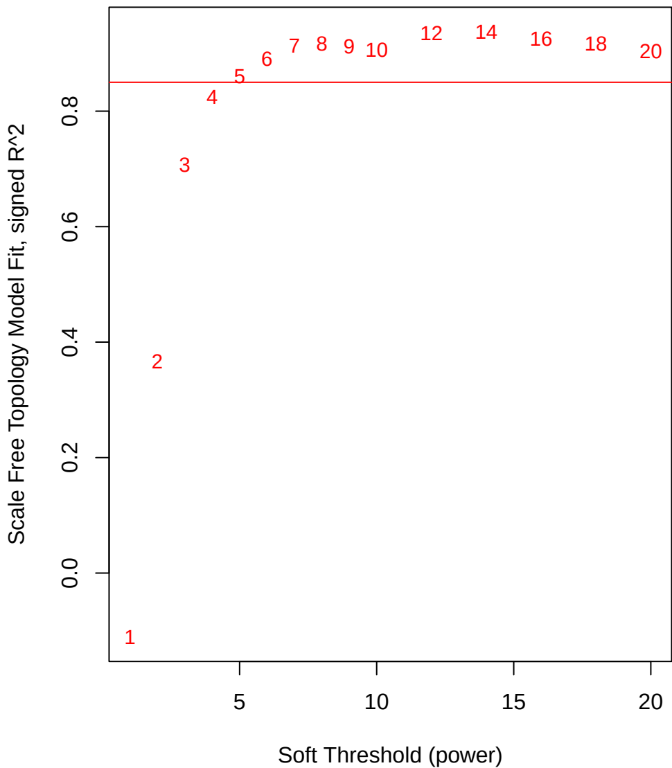
Scale independence
