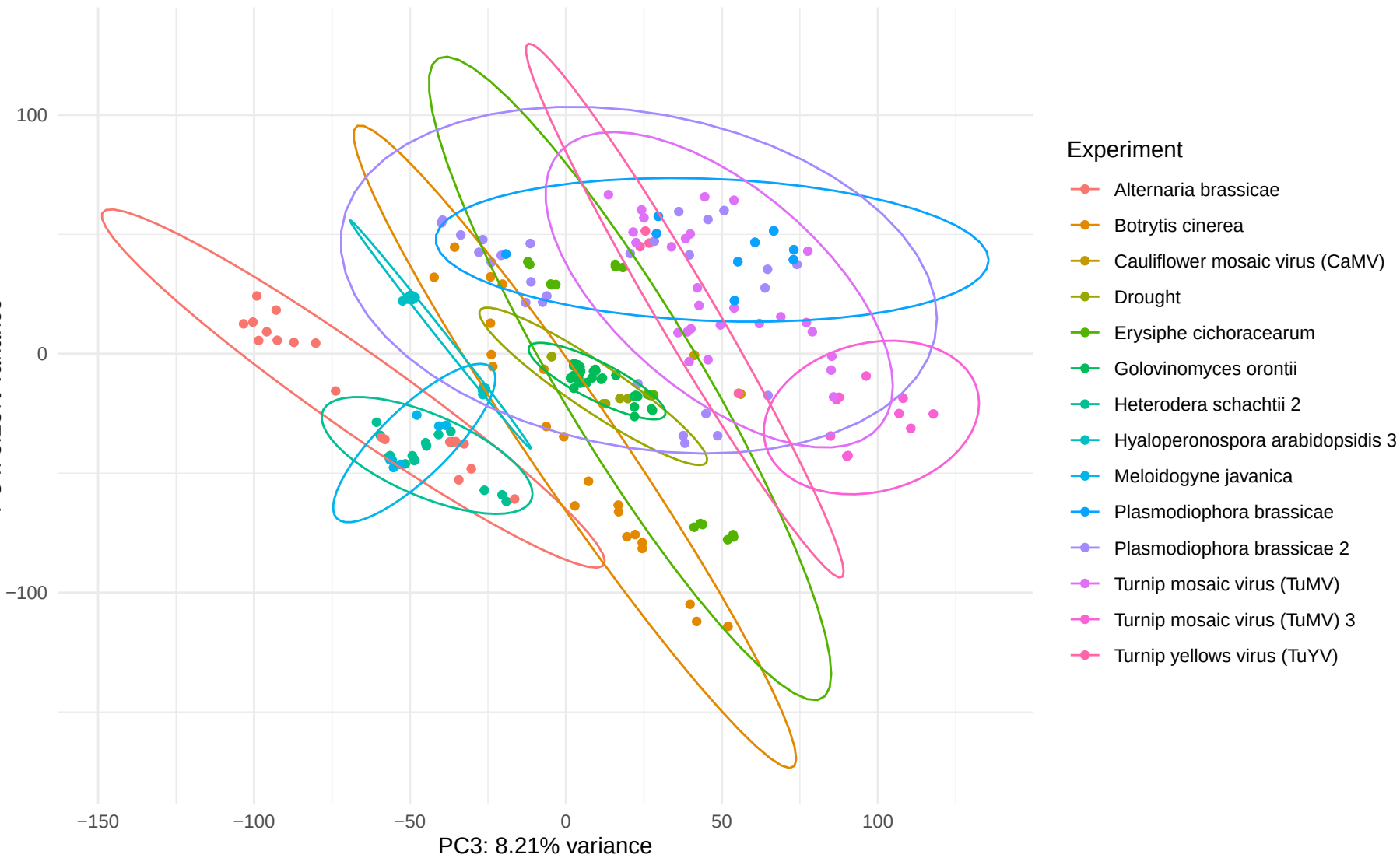
PCA of filtered vst counts
