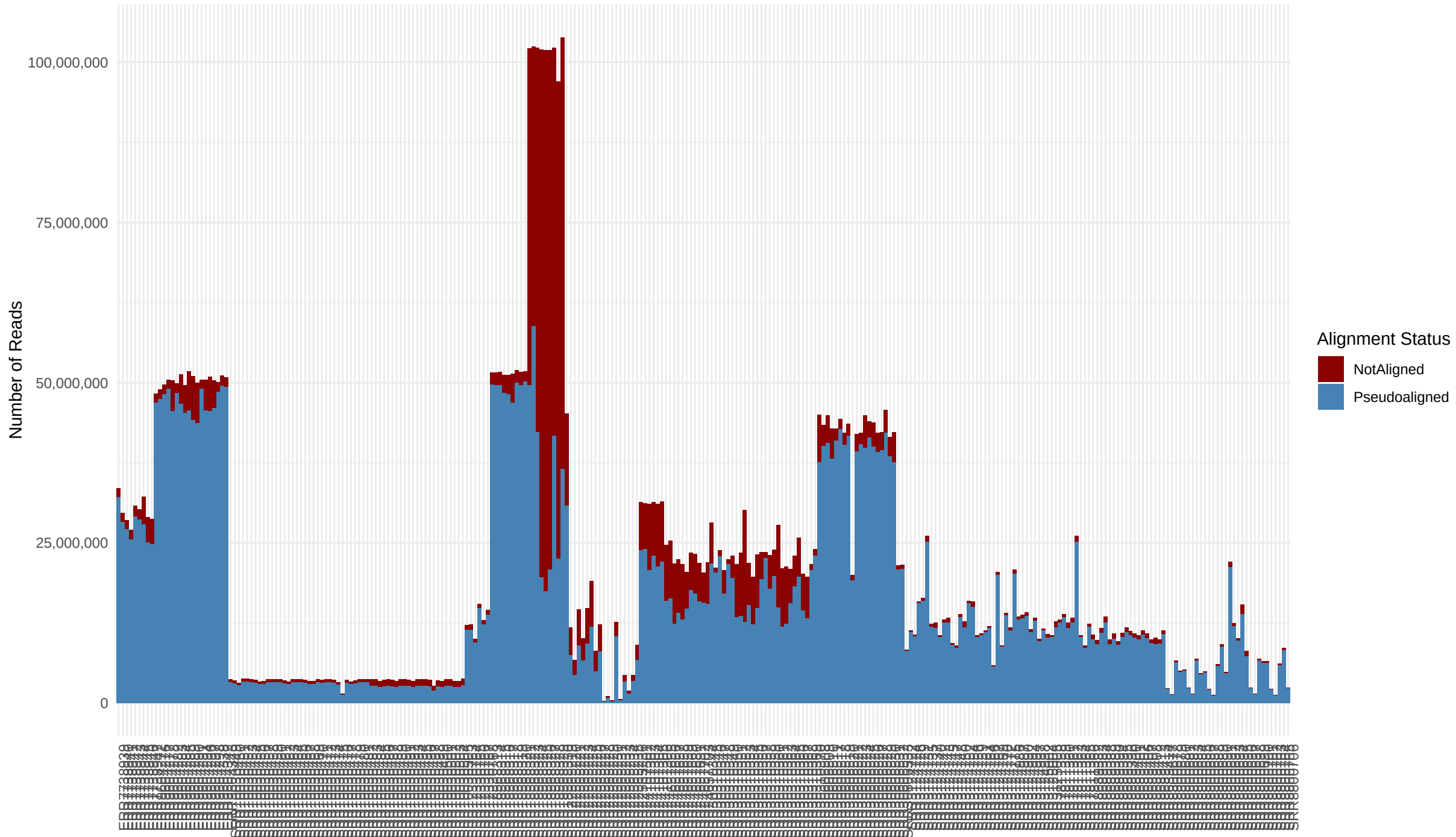
Kallisto: Alignment Scores for 283 samples
