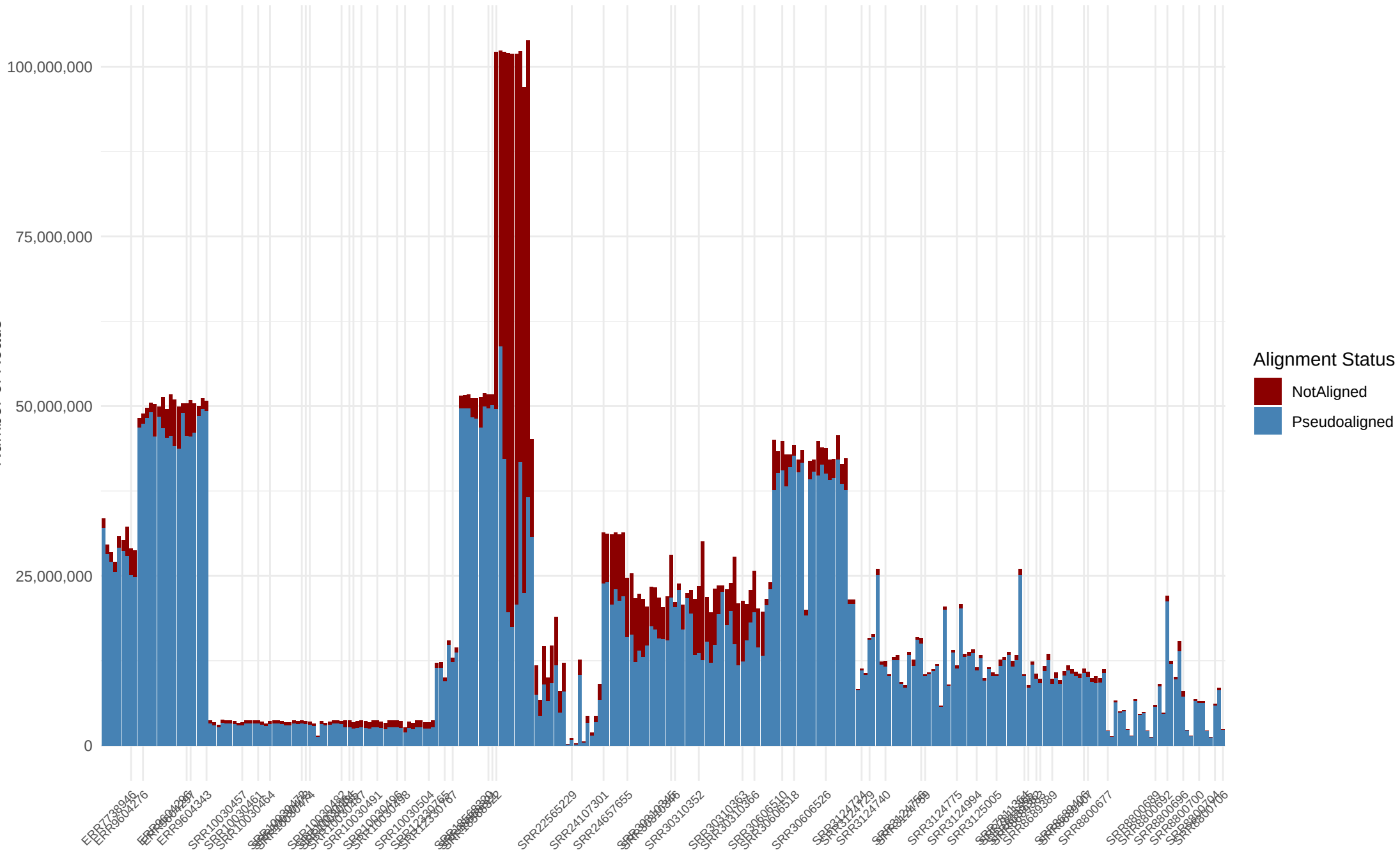
Kallisto: Alignment Scores for 283 samples
