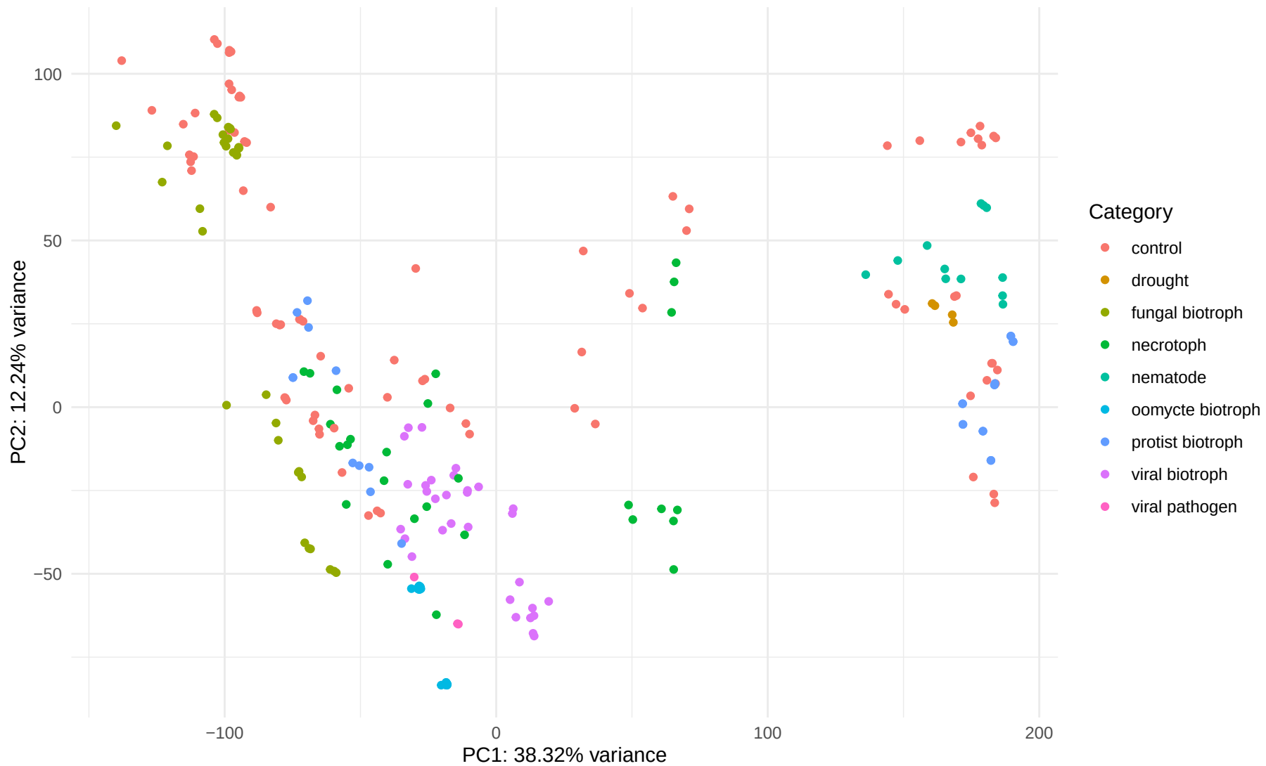
PCA of filtered vst counts – Pathogens (subcategories)
