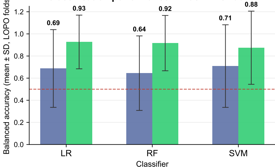
Classification performance — Task 1 vs Task 2
