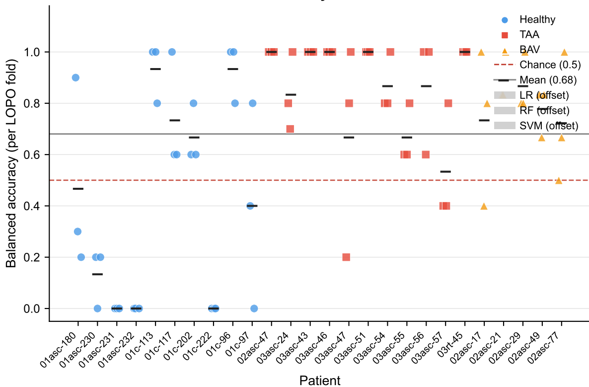
Task 1: Healthy vs Diseased
