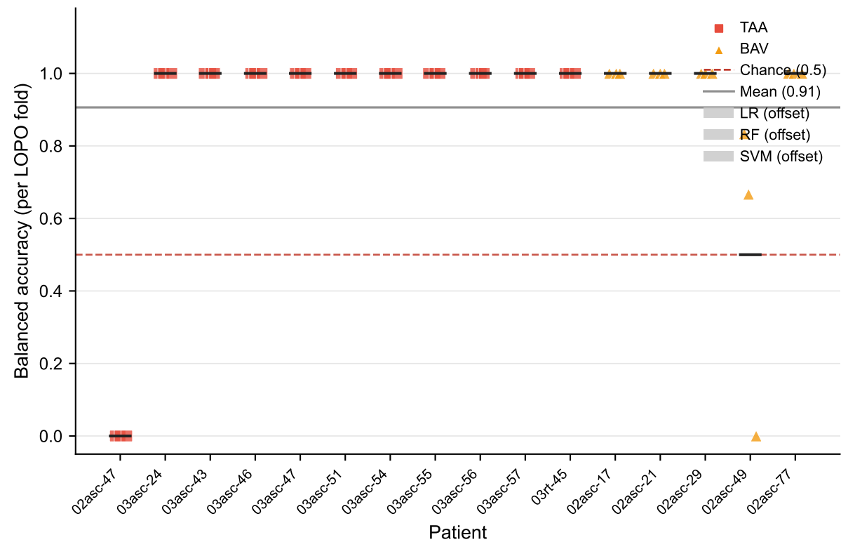
Task 2: TAV-ATAA vs BAV-ATAA
