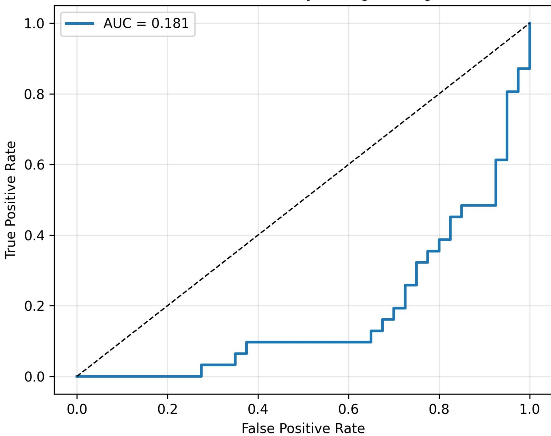
Task 1 — Diseased vs Healthy — LogisticRegression ROC
