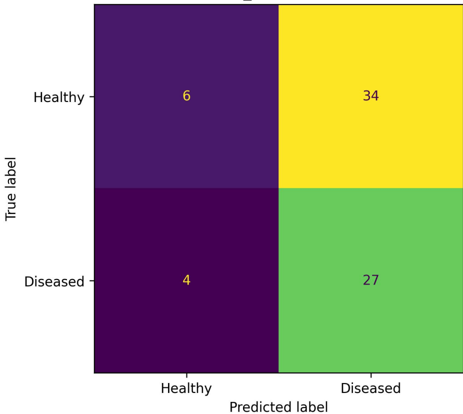
Task 1 — Diseased vs Healthy — RandomForest bal_acc=0.510
