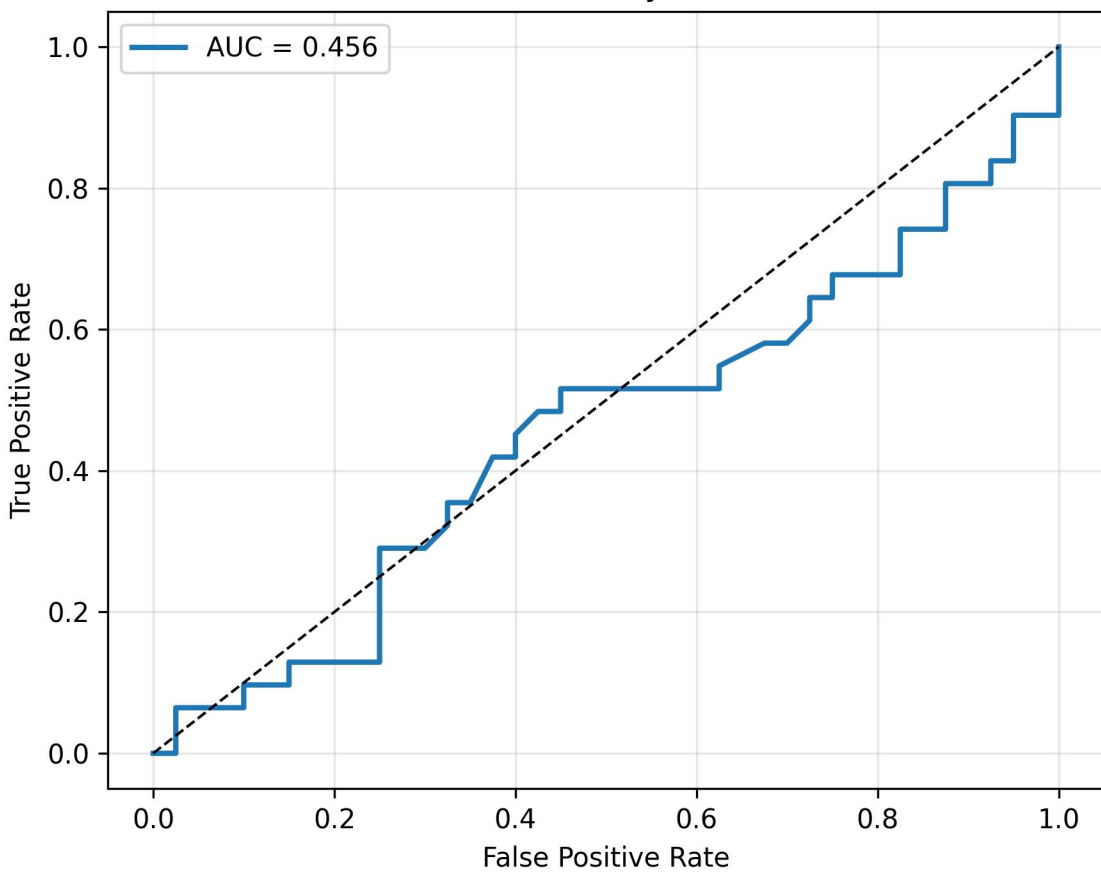
Task 1 — Diseased vs Healthy — RandomForest ROC
