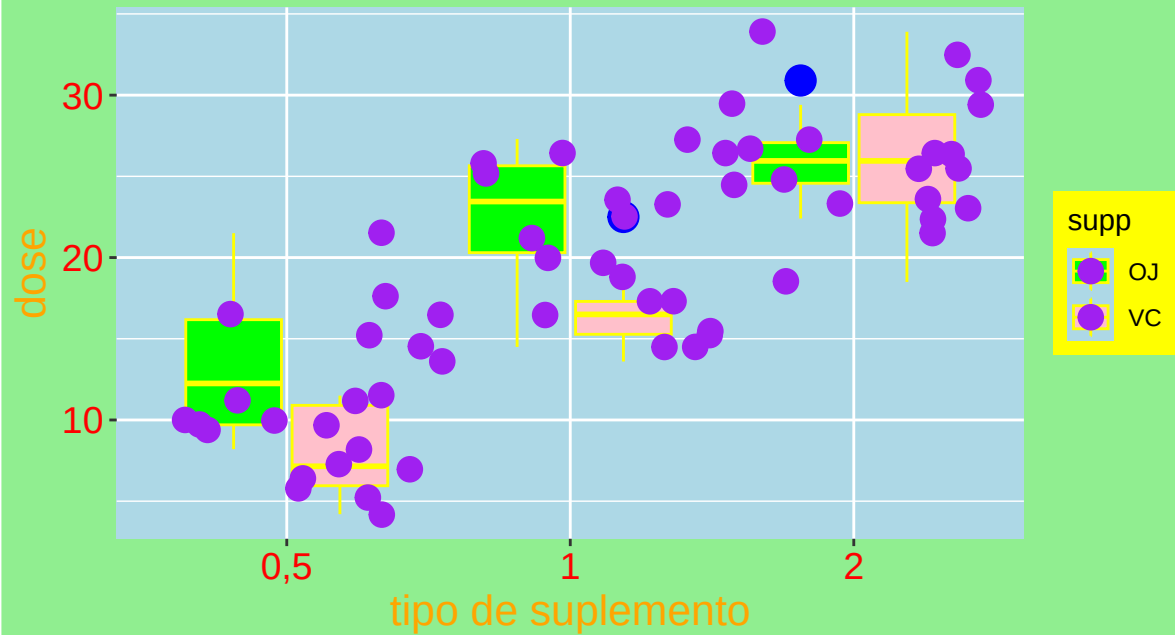
box plot
