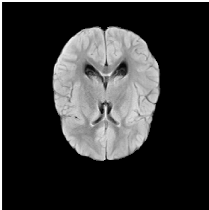
Ground Truth
