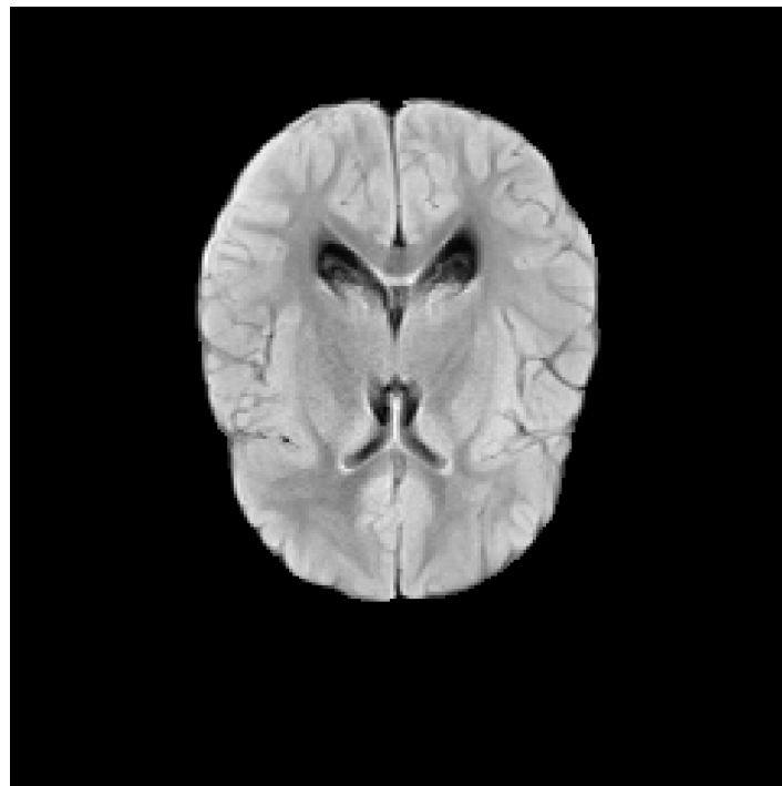
Baseline (Hard)
