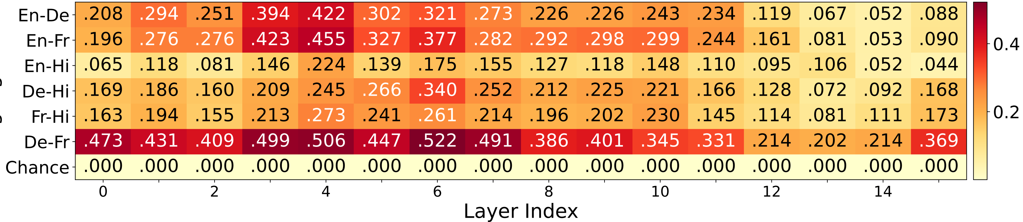
Top- k=0.0001
