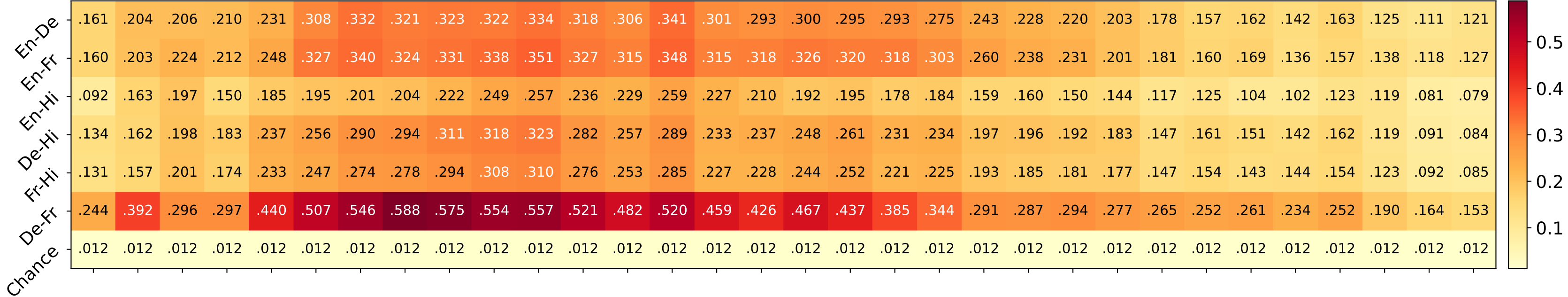
Top- k=0.025
