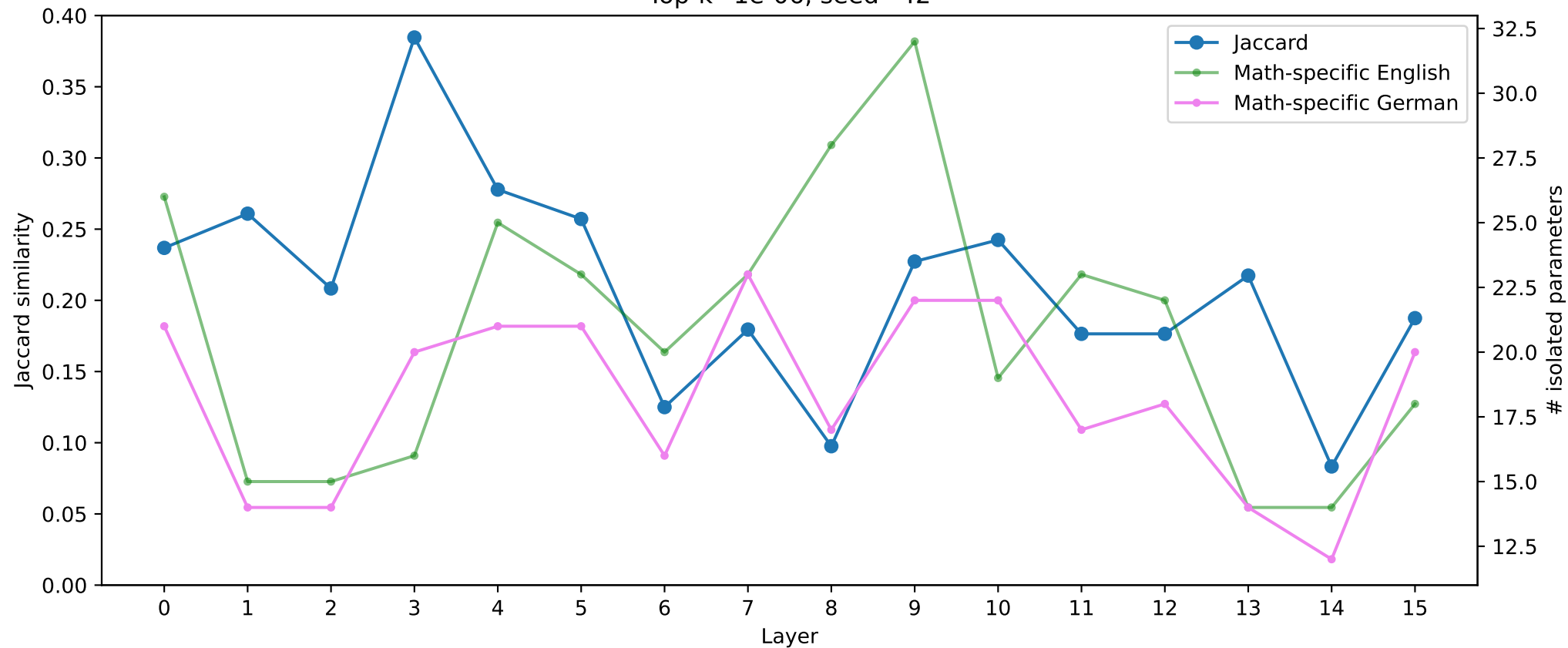
Top-k=1e-06, seed=42
