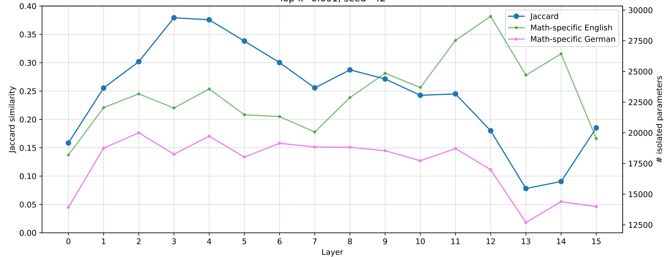
Top-k=0.001, seed=42
