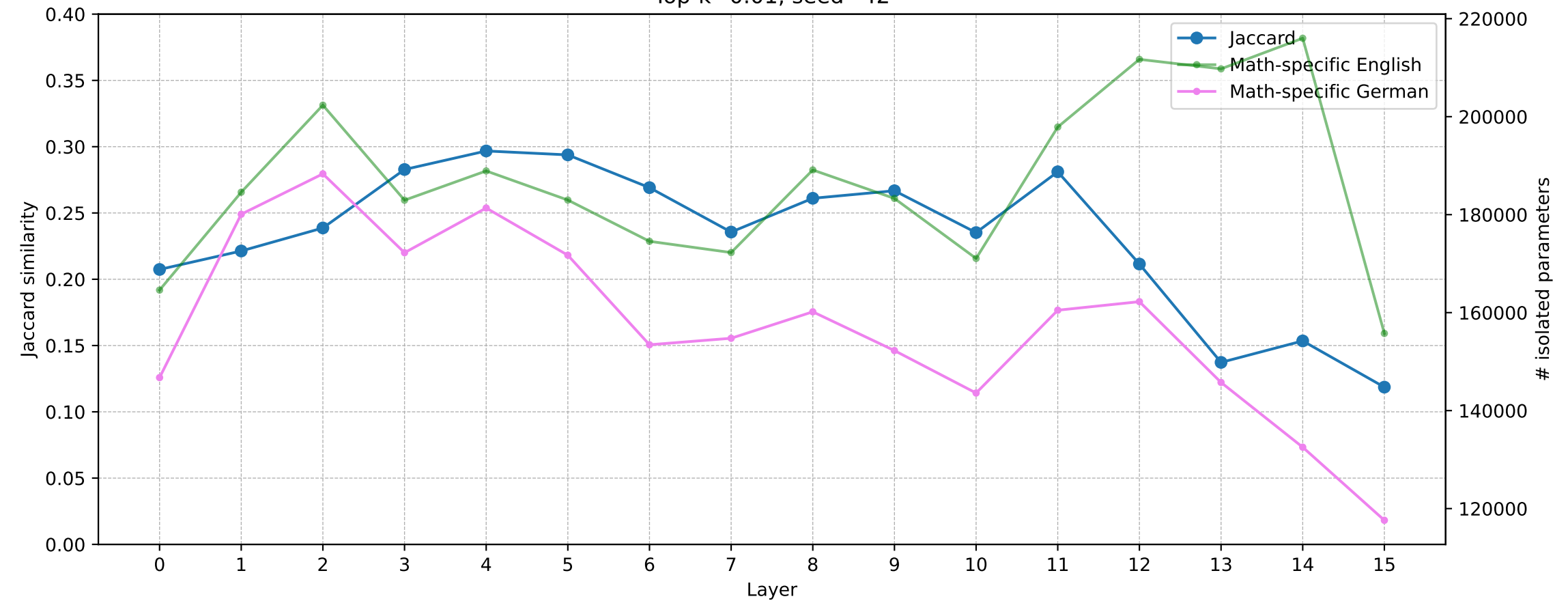
Top-k=0.01, seed=42
