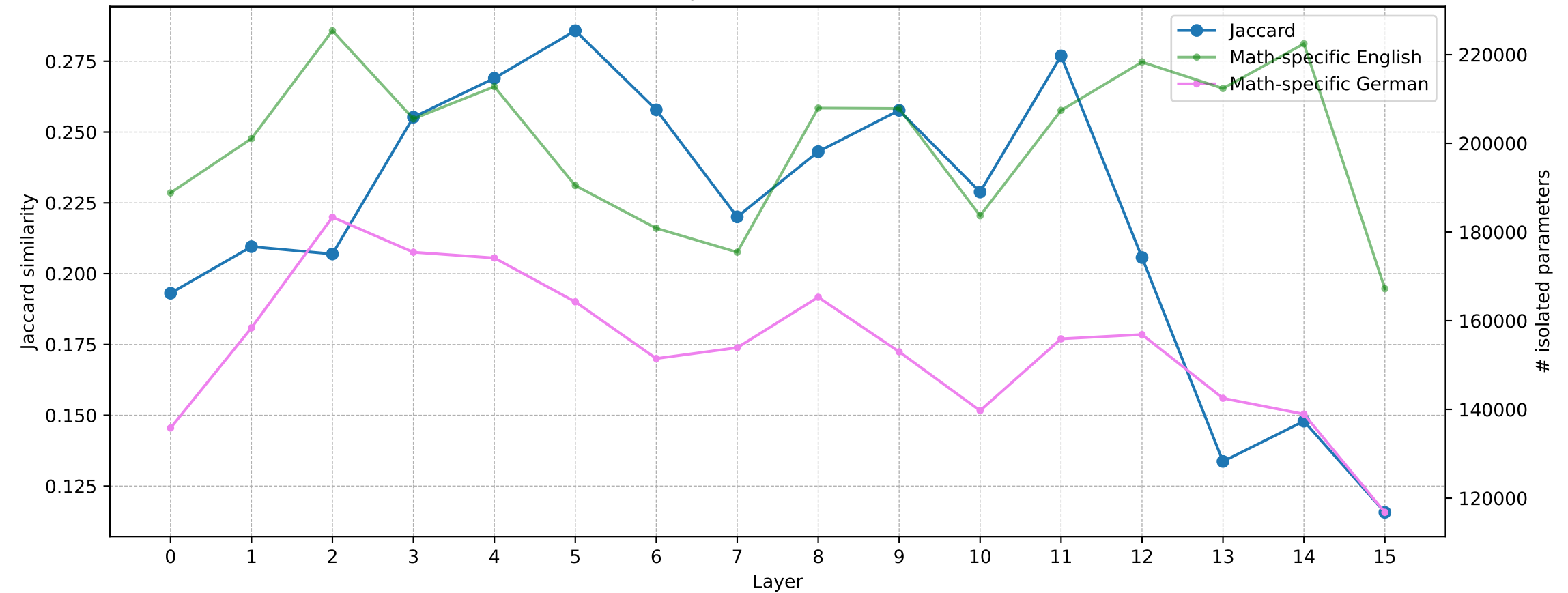
Top-k=0.01, seed=1
