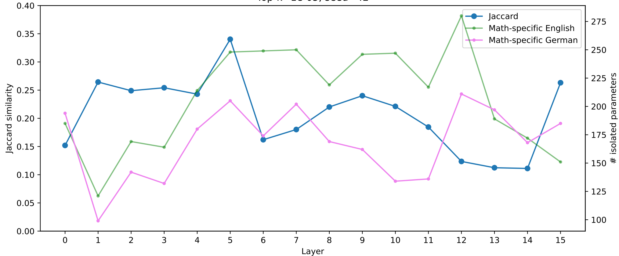
Top-k=1e-05, seed=42
