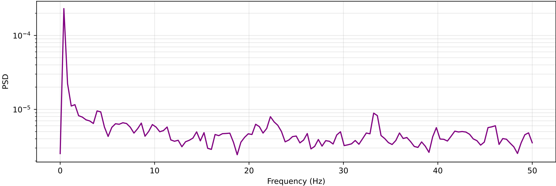
Combustion Stability (Pressure PSD) - Peak: 0.4 Hz
