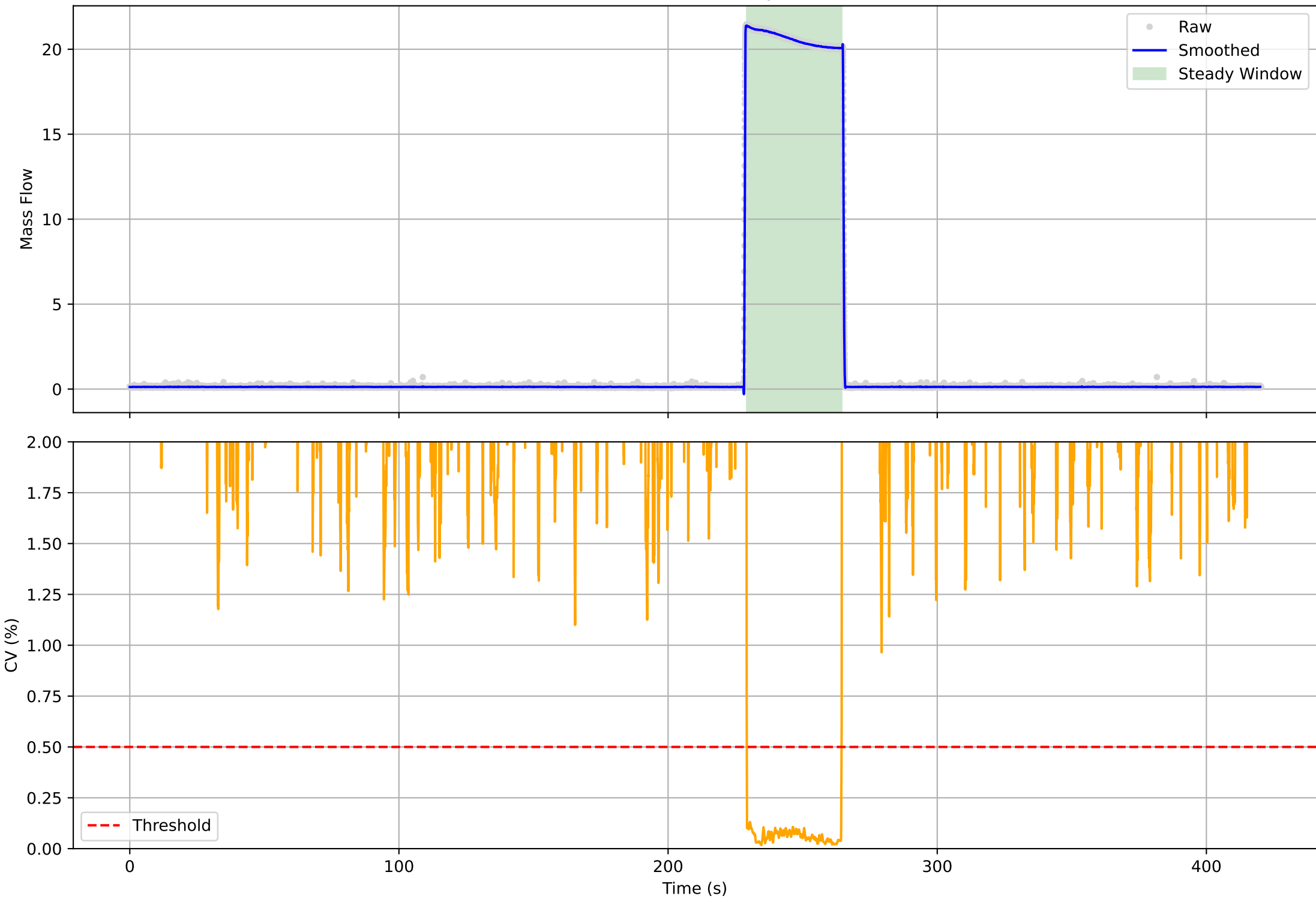
Detailed Flow Analysis
