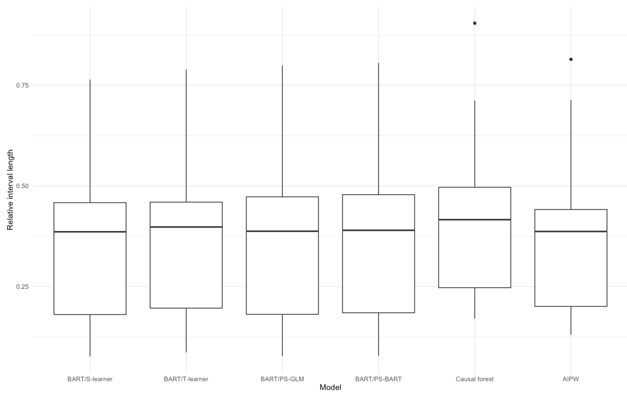
Abbildung .6: Distribution of relative interval length across DGPs by model
