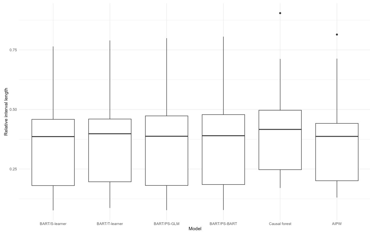
Abbildung .3: Distribution of relative interval length across DGPs by model
