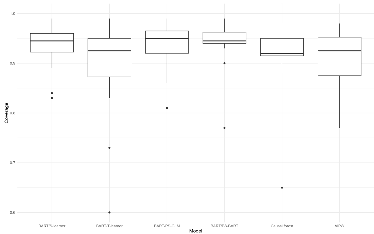
Abbildung .2: Distribution of relative coverage across DGPs by model (AIPW's outlier in DGP 30 excluded)
