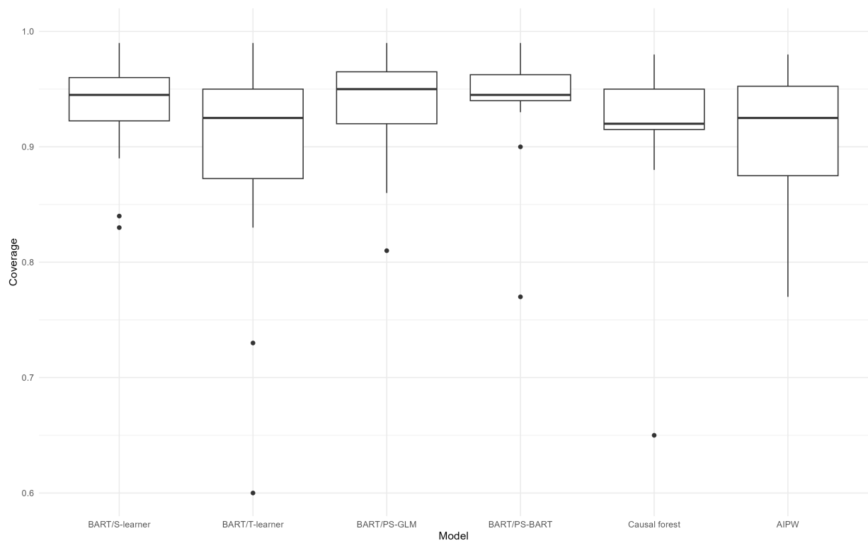
Abbildung .5: Distribution of relative coverage across DGPs by model (AIPW's outlier in DGP 30 excluded)
