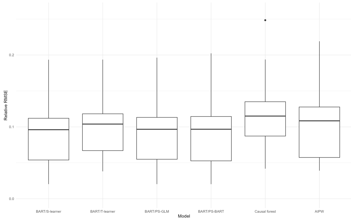
Abbildung .1: Distribution of relative RMSE across DGPs by model (AIPW's outlier in DGP 30 excluded)
