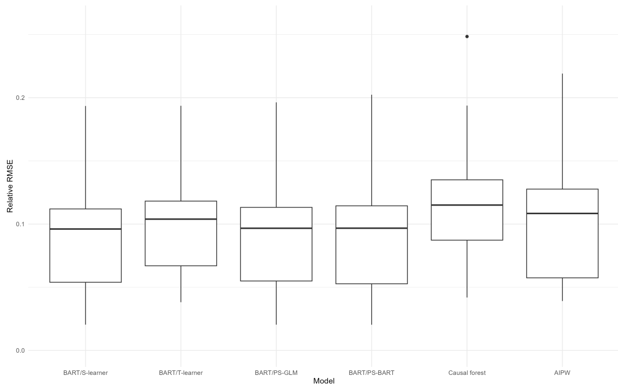
Abbildung .4: Distribution of relative RMSE across DGPs by model (AIPW's outlier in DGP 30 excluded)
