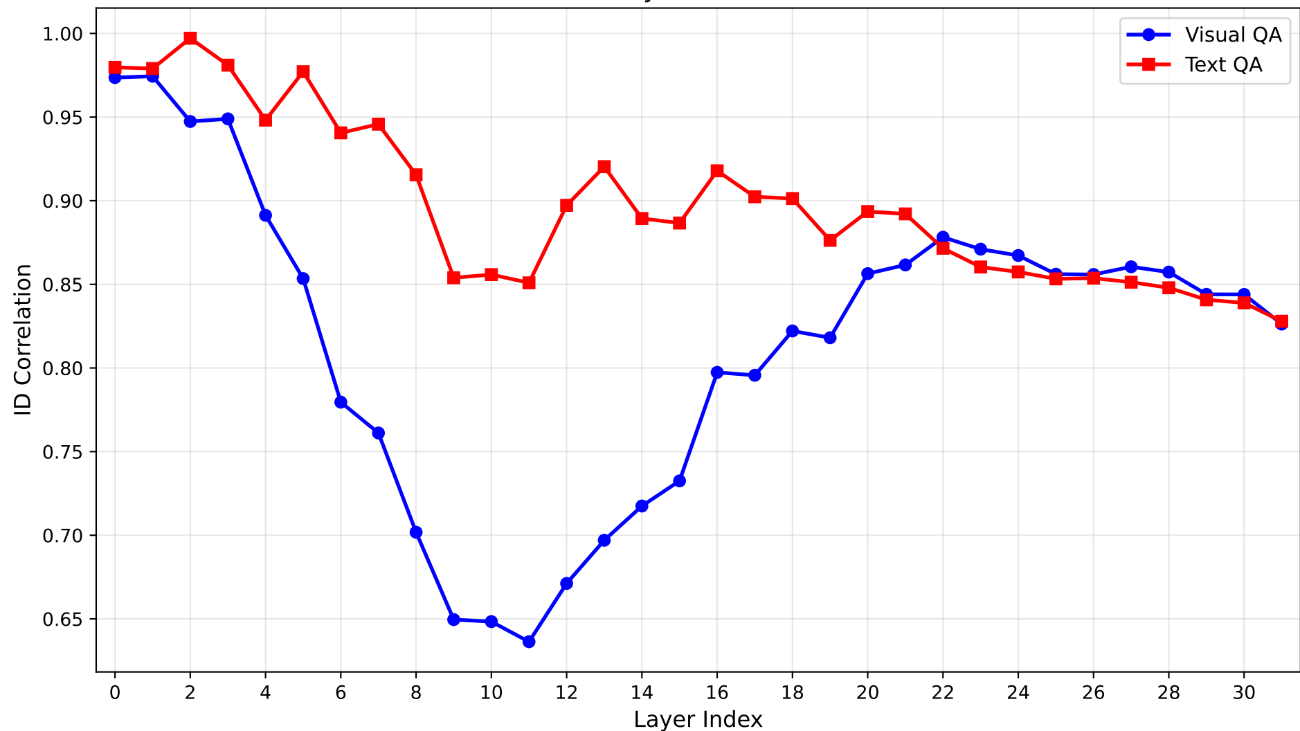
ID Correlation Across Layers: LLaVA-1.5-7B vs Vicuna-7B
