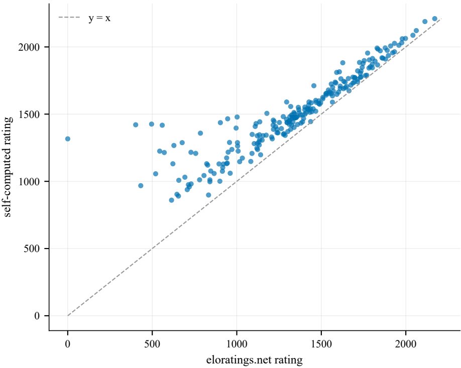
Self-computed vs eloratings.net (latest per team)
