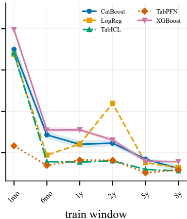
Train-size ablation — one-step (tuned classical vs tune-free FM) few features best features
