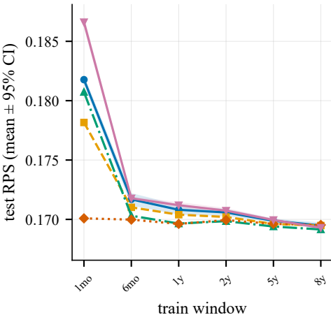
Train-size ablation — one-step (tuned classical vs tune-free FM) few features best features
