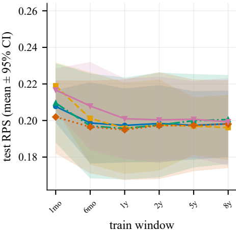
Train-size ablation — multi-step Cup-match RPS (tuned classical vs FM)
