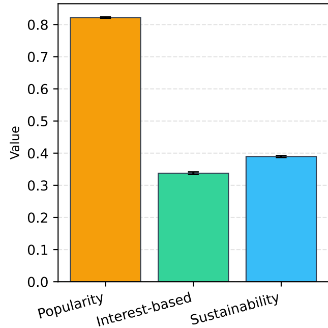
Recommender strategy comparison (sustainability mission scenario, mean \pm std, 4 seeds)
