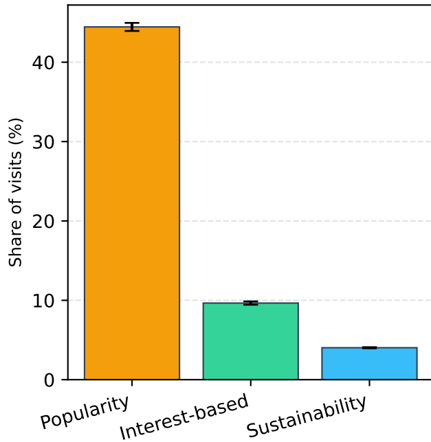
Recommender strategy comparison (sustainability mission scenario, mean \pm std, 4 seeds)
