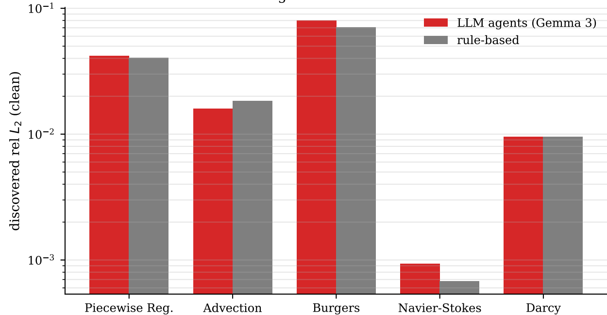
Ablation: LLM-agent vs. rule-based coordination
