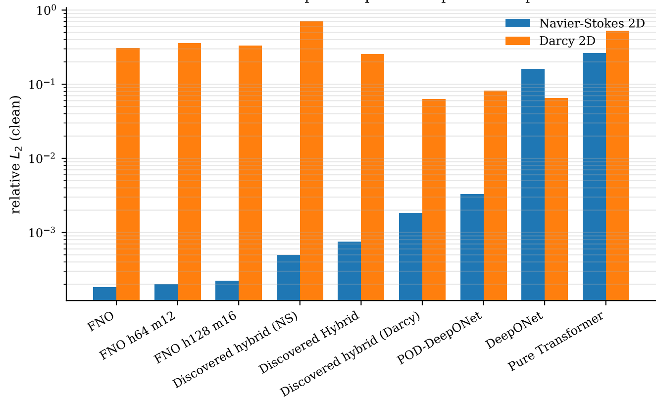
No universal winner: optimal operator is problem-dependent
