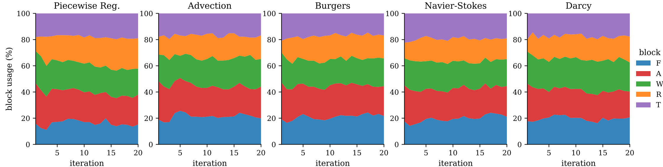
Maintained diversity: population block-usage stays mixed (no groupthink collapse)
