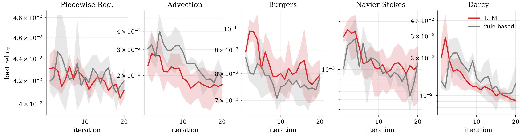
Swarm convergence: LLM agents vs. rule-based (mean \pm s.d. over seeds)
